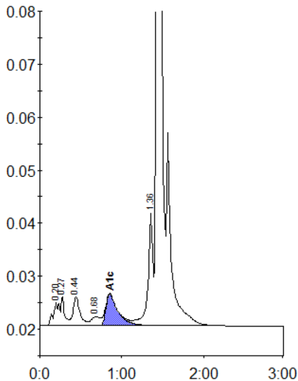
Peak table - ID: 10558011
